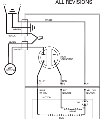
WIRING DIAGRAM FOR MODELS WD4405 ALL REVISIONS
