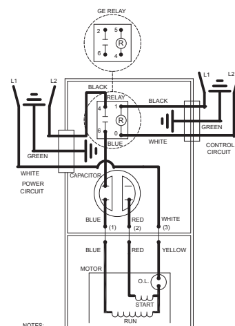
WIRING DIAGRAM FOR MODELS XE4405 ALL REVISIONS
