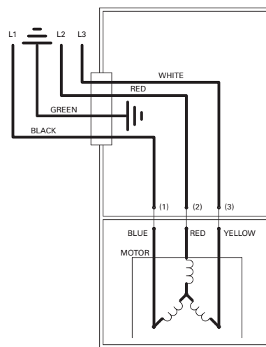
WIRING DIAGRAM FOR MODELS J4404, F4404, G4404 AND BA4404 ALL REVISIONS
