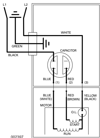
WIRING DIAGRAM FOR MODELS E4404 AND I4404 ALL REVISIONS
