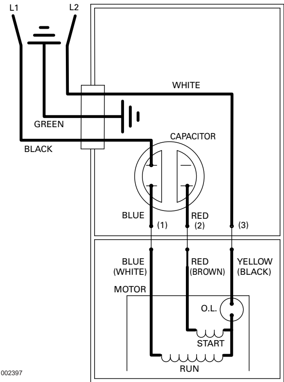
WIRING DIAGRAM FOR MODELS "E191" 6/95 thru Current
