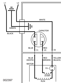
WIRING DIAGRAM FOR MODELS E405 & I405 ALL REVISIONS
