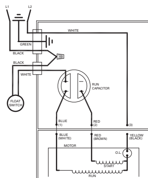
WIRING DIAGRAM FOR MODEL WD405 ALL REVISIONS
