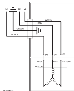
WIRING DIAGRAM FOR MODELS J405, F405, G405 AND BA405 ALL REVISIONS
