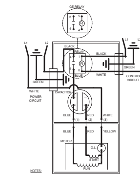
WIRING DIAGRAM FOR MODEL XE405 ALL REVISIONS
